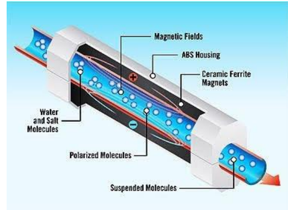
Fig. 4: Magnetic water conditioner
