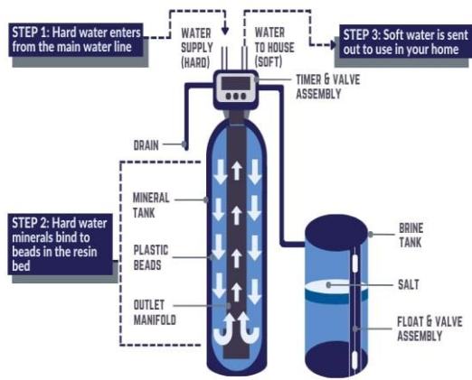
Fig. 2: Ion Exchange process
